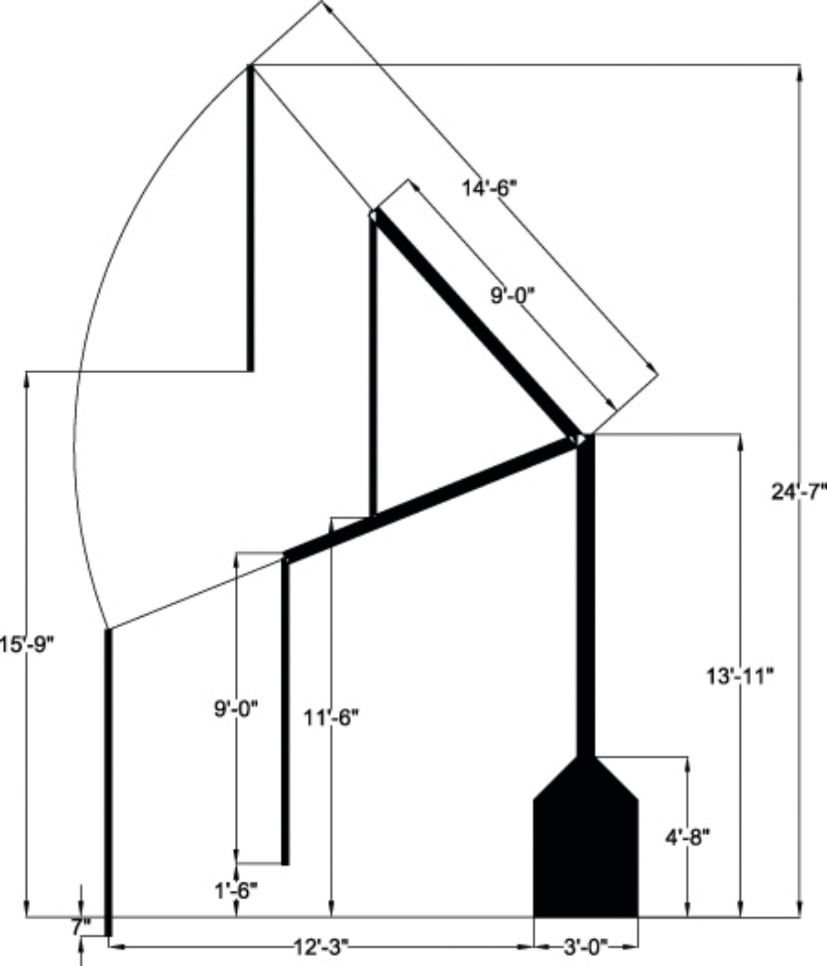
CR Manufacturing Shuttle II Grain Probe Clearance Dimensions
